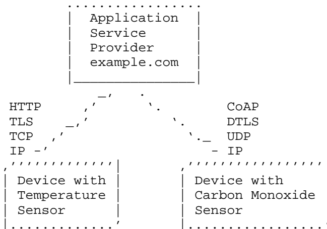
Figure 2: Device-to-Cloud Communication Pattern
